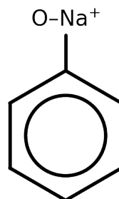
sodium phenoxide
