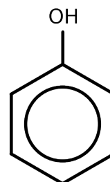
phenol
