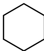
cyclohexane
