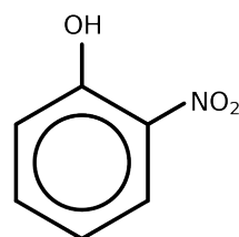
2-nitrophenol
