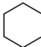
cyclohexane
