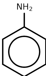
phenylamine
