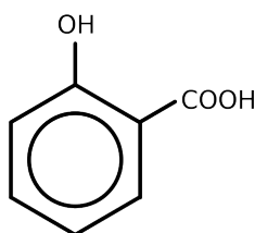
2-hydroxybenzoic acid
