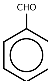
benzaldehyde
