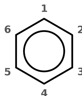
phenol
