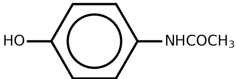
paracetamol
