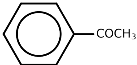
phenylethanone
