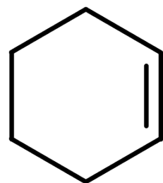
cyclohexene
